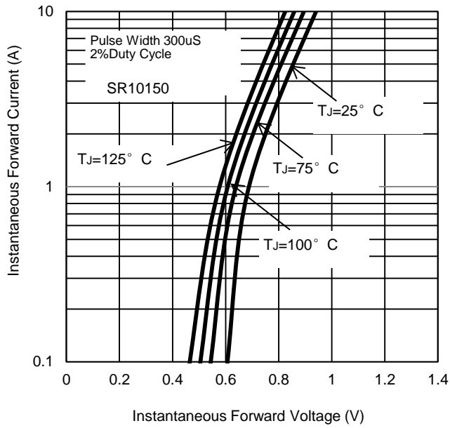
Fig. 7 - Typical Forward Characteristics
